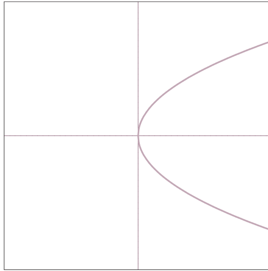
Abbildung 4.7: Parabel x_1 - x_2^2 = 0 in \mathbb{R}^2 .
